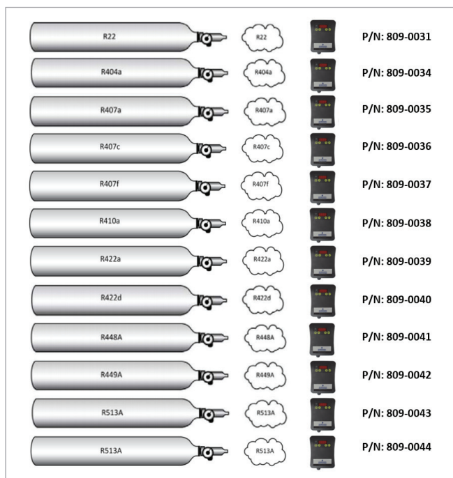
Gas-Specific MRLDS-250 Gas Detectors
